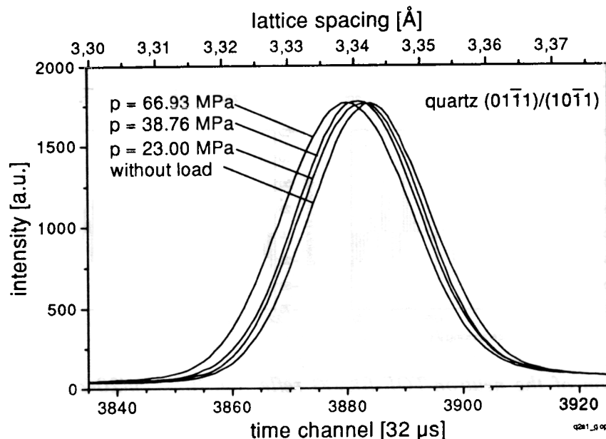
Fig. 4: Peak shift as a function of applied stresses up to about 67 MPa demonstrated with the (01-11)/(10-11) BRAGG reflection of quartz.
